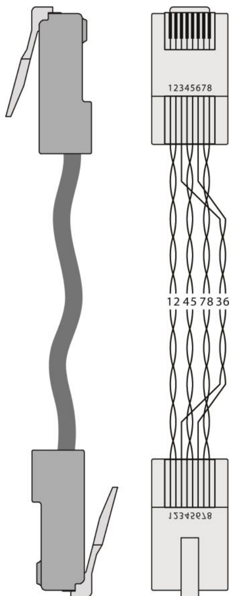
Figure 7: TP PINOUT
