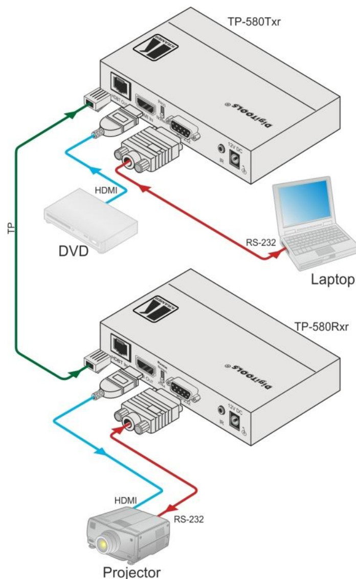
Figure 6: RS-232 Control
